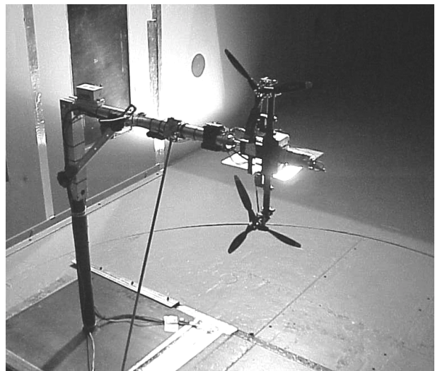
Fig. 1. Tiltrotor Descent Aerodynamics test in the Ames 7- by 10- Foot Wind Tunnel.
