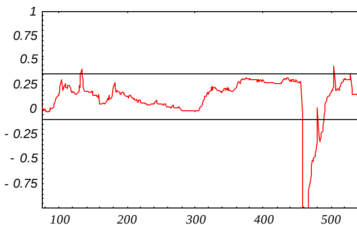
Figure 3. Cuscore statistic showing blower failure detection.
