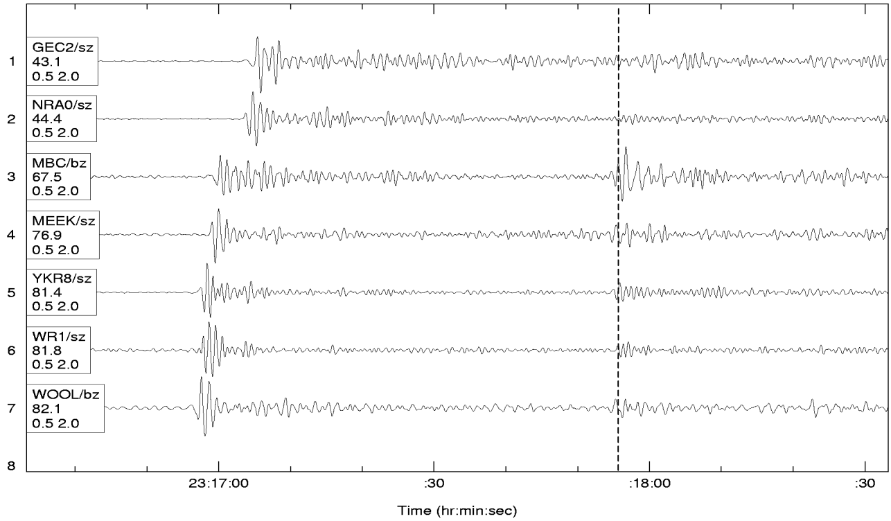
Figure 6. Vertical component teleseismic recordings of the Hindu Kush earthquake of 1995/08/17, shown aligned on the candidate pP phase arrival time identified by the network stacking algorithm. The annotated numerical values on each trace denote the relative amplitudes of P and pP to be used as input to the Pearce focal mechanism code RAMP.
