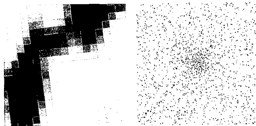
Fig. 7. Left panel: the IRAS 100 \mu m map of the field around IC 361. Right panel: the cluster image in DSS2 Red. Both maps have the same center and the same size, 25' \times 25' .
