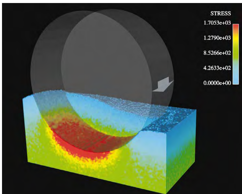
FIGURE 2. WHEEL OF MINE PLOW. Pictured is an idealized wheel, rendered partially transparent, turning into a 10 million particle soil mass in the direction of the arrow. Colors indicate stress exerted on individual particles in the soil from blue (low) to red (high).
