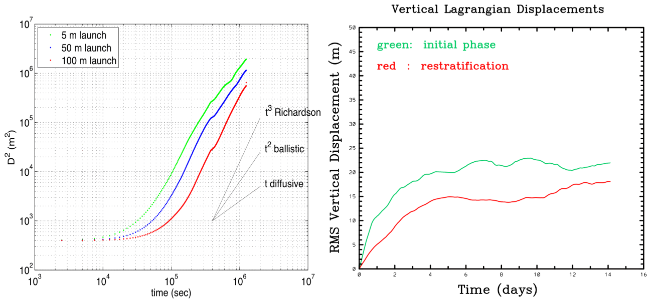
Fig. 7: (Left panel) Relative dispersion from particles launched at three depth levels. (Right panel) Rms vertical displacement from particles during different dynamical phases of the mixed layer instability.
