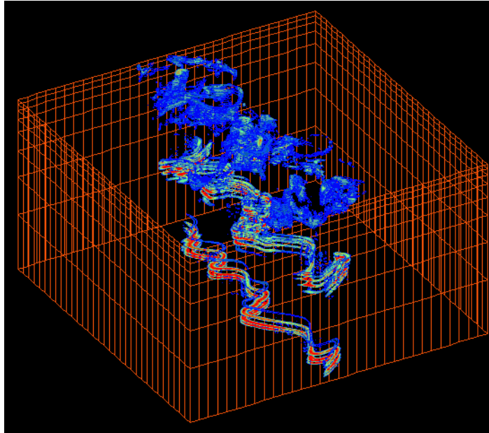
Fig. 5: Snapshot of the tracer field (for non-dimensional concentration > 0.1 ) at 10 days after being released at three depth levels during the mixed layer instability.
