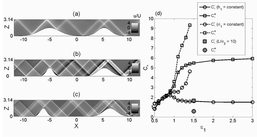
Figure 1: (a)-(c) Internal tides radiated by different configurations of a double ridge system. A small shift in the position of the left ridge (i.e. (b) compared to (c)) creates a substantial difference in the radiated wave field. (d) The dimensionless energy-flux as a function of the criticality of the left ridge. There is a distinct asymmetry between the left- ( C^- ) and right-going ( C^+ ) energy flux.
