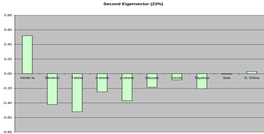
Figure 5. Second principle component of strait transport, wind stress, and sea-level.
