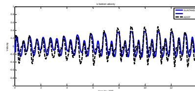
bottom u-velocity
