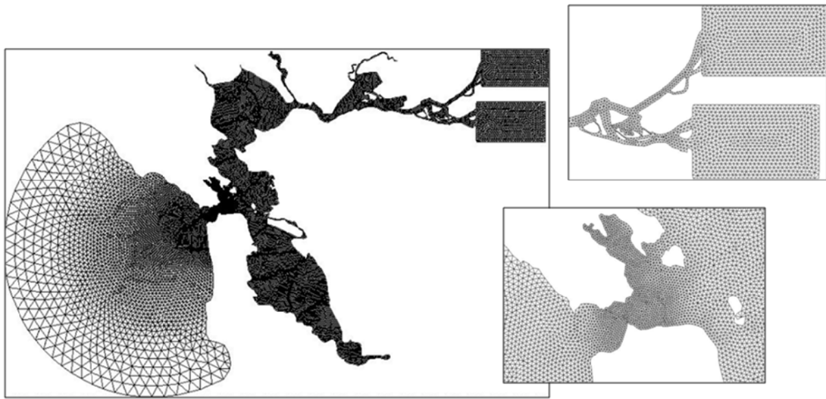
Figure 1: Coarse full-Bay grid with an average 200 m resolution throughout the Bay.
