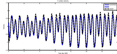
surface v-velocity
