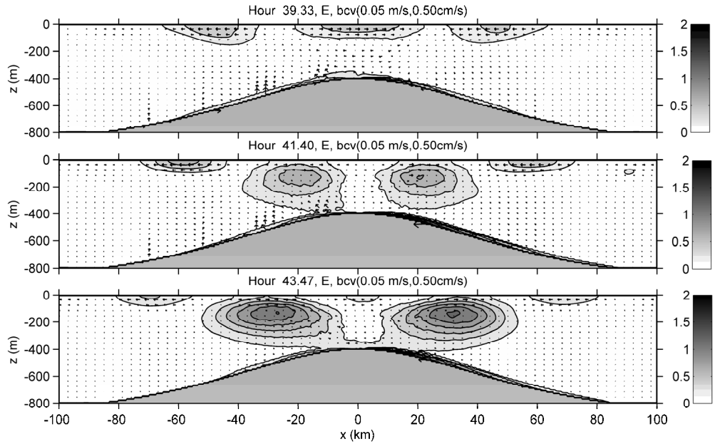
Figure 2. Same as Figure 1 but for ridge half-width L = 60 km. The contour interval is 0.2 J/m^3 . A vector of size of the grid box is 0.05 m/s and 0.5 cm/s in the horizontal and vertical directions, respectively.
