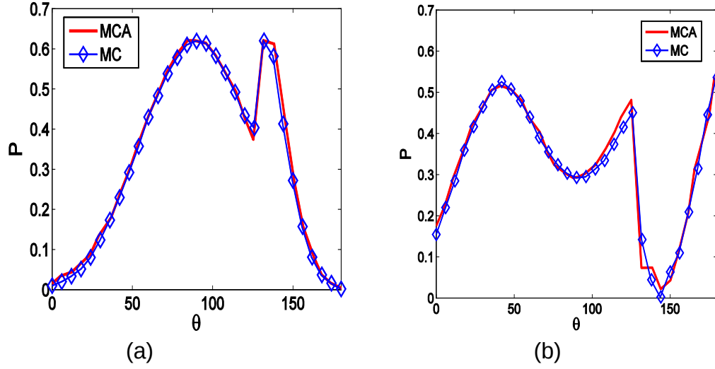
Figure 1: Comparisons of the present Monte Carlo RT simulation (blue line with symbols) with the prediction by the Multi-Component Approximation method (red line). The plotted is the averaged degree of polarization as a function of polar angle \theta observed at optical depth cz = 0.01 , for incident sun with (a) zenith angle \theta_s = 0^\circ and azimuth angle \phi_s = 0^\circ ; and (b) \theta_s = 60^\circ and \phi_s = 0^\circ .
