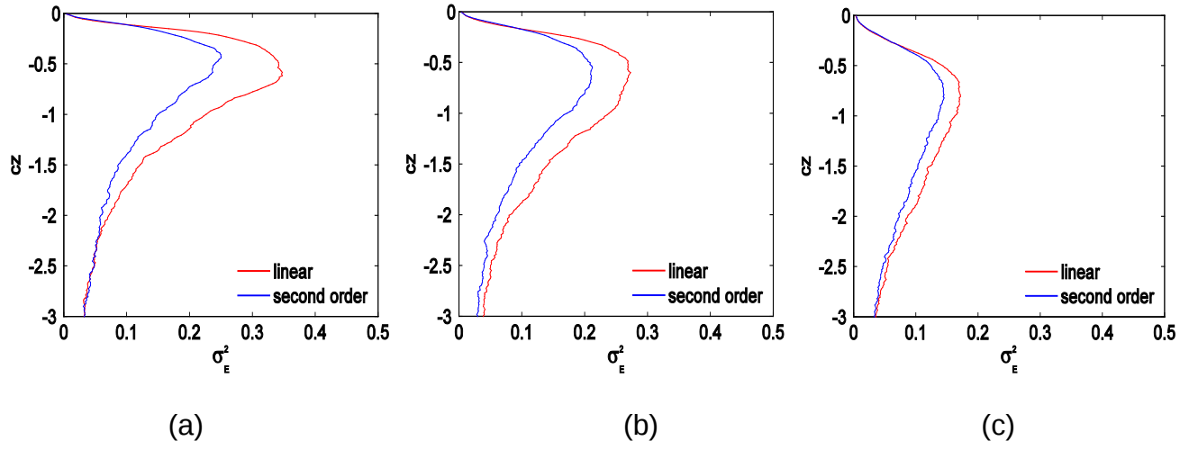
Figure 3. Dependence of underwater irradiance variance ( \sigma^2 ) at various optical depth ( cz ) on surface wave steepness: (a) wave steepness k_p A_p = 0.30 , (b) k_p A_p = 0.20 , and (c) k_p A_p = 0.10 . The results are obtained with the ocean surface wave given by the linear wave theory (red line) and the nonlinear wave theory including the second-order wave effects (blue line).
