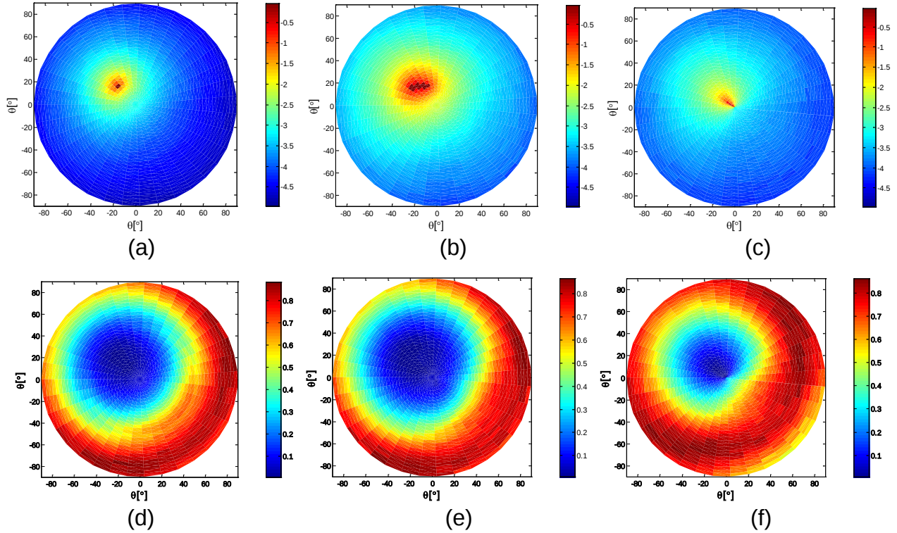
Figure 2. Vector radiance I(\theta) (top: a, b, c) and averaged degree of polarization P(\theta) (bottom: d, e, f) under flat surface (left: a, d), regular waves (middle: b, e) and irregular waves (right: c, f), received at optical depth cz = 1.0 under the mean ocean surface. Incident sun has zenith angle \theta_s = 30^\circ and azimuth angle \phi_s = 135^\circ .
