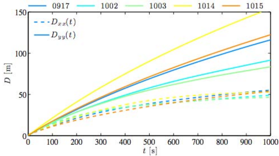
Figure 5: Growth of tracer patch size D versus time, estimated from drifter data. Initially, D=0 . Solid and dashed lines are the along-shore ( y ) and cross-shore ( x ) patch dimensions, respectively. Colors correspond to different days during HB06 (from Spyde et al, 2009.)
