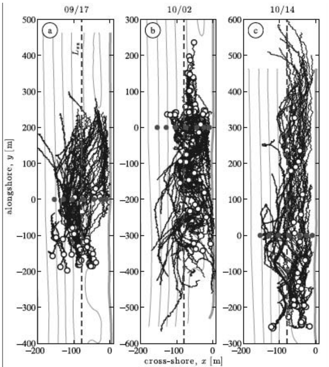
Figure 4: Drifter trajectories (black curves) for 3 days during HB06. Open circles are drifter release locations. Individual drifters moved as much as 600m alongshore, but less than 100m offshore.
