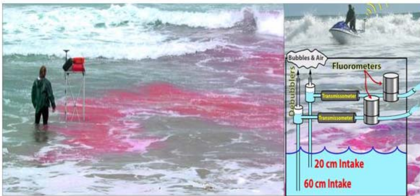
Figure 1 (left) tracer dye injected continuously into the surfzone at a controlled rate forms a plume (right) GPS-tracked, dye-sampling jet ski on a transect across the surfzone. On-board, flow-through dye sampler (inset) includes an electric pump, a debubbler, a turbidity sensor, and a Rhodamine WT dye fluorometer, sampling at 5Hz. To reduce effects of bubbles and sand on the optically measured dye concentration, the jetski is driven in the relatively low turbulence region in front of a bore. A handlebar-mounted screen displays realtime data and a local position map, allowing repeated sampling of pre-determined transects. Position and sensor data are transmitted ashore, allowing real-time analysis and adaptive sampling.
