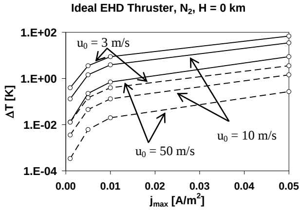
Fig. 14. An estimation for \Delta T_q ; solid lines: L = 1\text{m} , dashed lines L = 10\text{cm}
