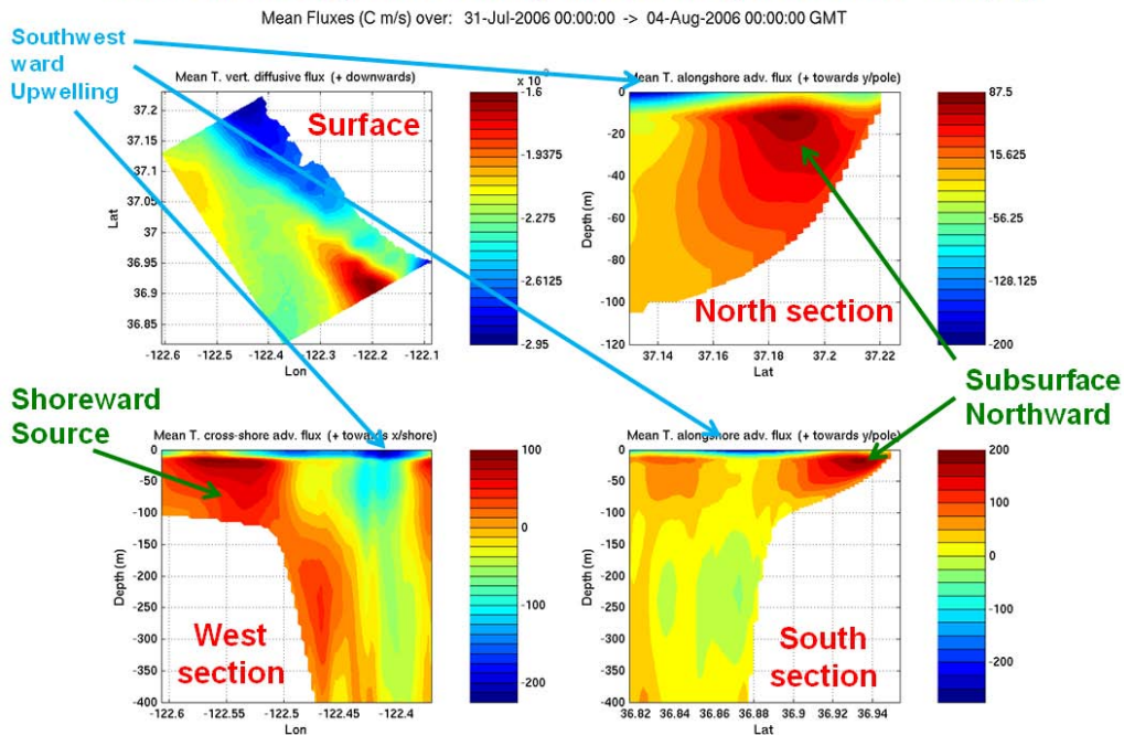
Figure 4. Advective and diffusive temperature fluxes through the boundaries of the control volume, averaged over the 4 days of the first upwelling event of MB06.
