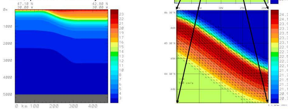
Figure 1. Idealized test case for testing 2-way nesting algorithms.
