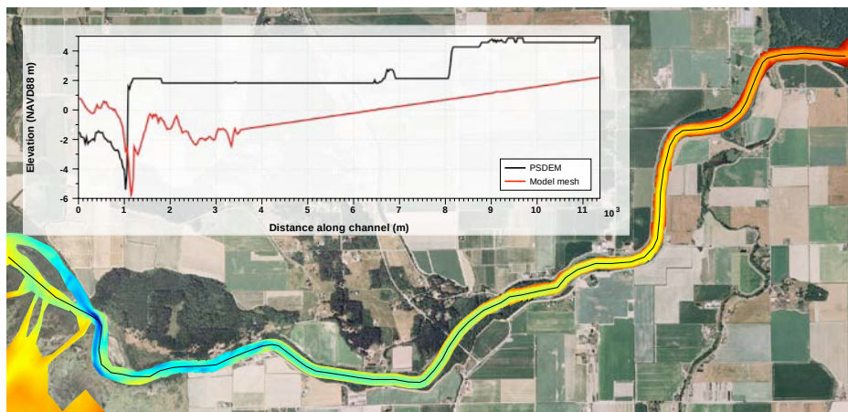
Figure 4: Channel depth shaded, with profile along the centerline of the channel. Inset figure shows the original DEM elevation, and the profile after adjustment and incorporation of Areté’s soundings. Note the >2 m drop in the DEM channel, which caused significant model instability.
