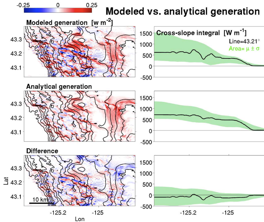
Figure 5: Left: spatial patterns of barotropic to baroclinic conversion, as assessed from the divergence of the baroclinic energy flux (top). This is compared to Nycander's (2005) analytical formation (middle). The difference (bottom) is mostly associated with high-k generation, so averages to zero in cross-slope integrals (right).
