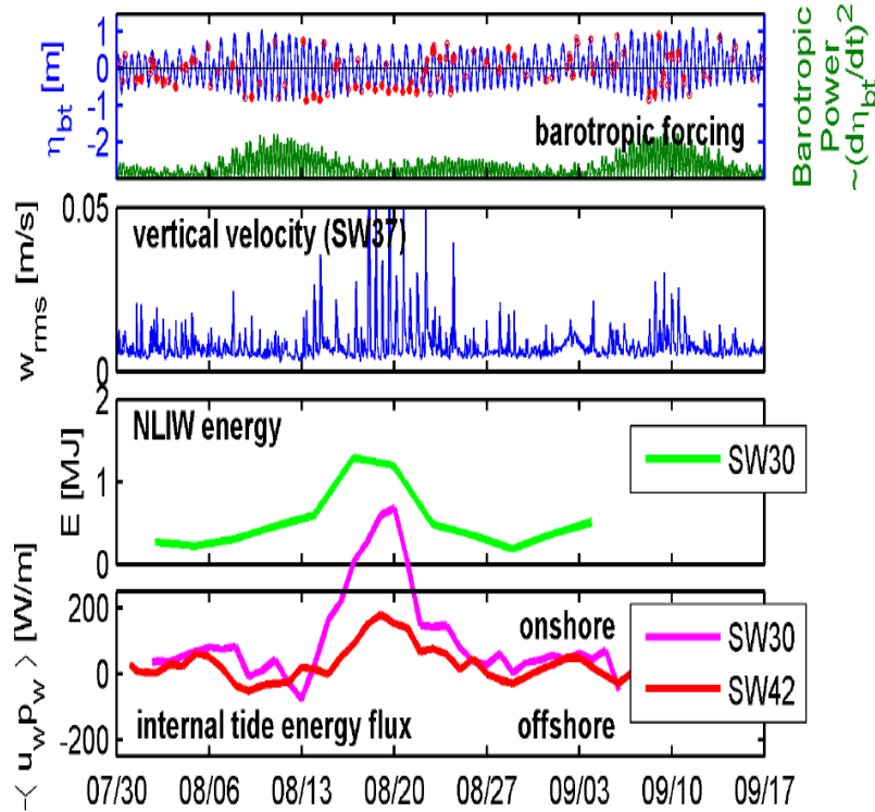
Figure 1: Summary of NLIW temporal variability. Forcing by the barotropic tide (elevation & power; top row) is poorly correlated with NLIW vertical velocity at SW37, the 70-m isobath (2 nd row). Red dots in upper panel represent wave arrival times at SW37. The resultant NLIW energy (3 rd row) is found to covary with the internal tide energy flux, both inshore and at the shelfbreak (bottom row).
