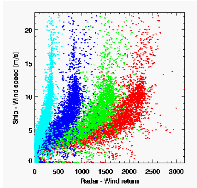
Figure 3: Scatter plot of the average radar return in four different range sectors determined from Knorr imagery collected in the period from August 14 to September 13, 2006.
