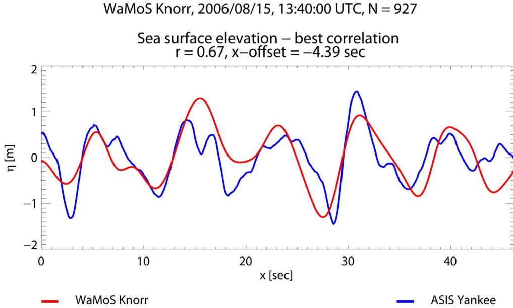
Figure 2: Correlation between surface elevation data from the wavestaffs of ASIS Yankee buoy and the inverted marine radar backscatter onboard the R/V Knorr.
