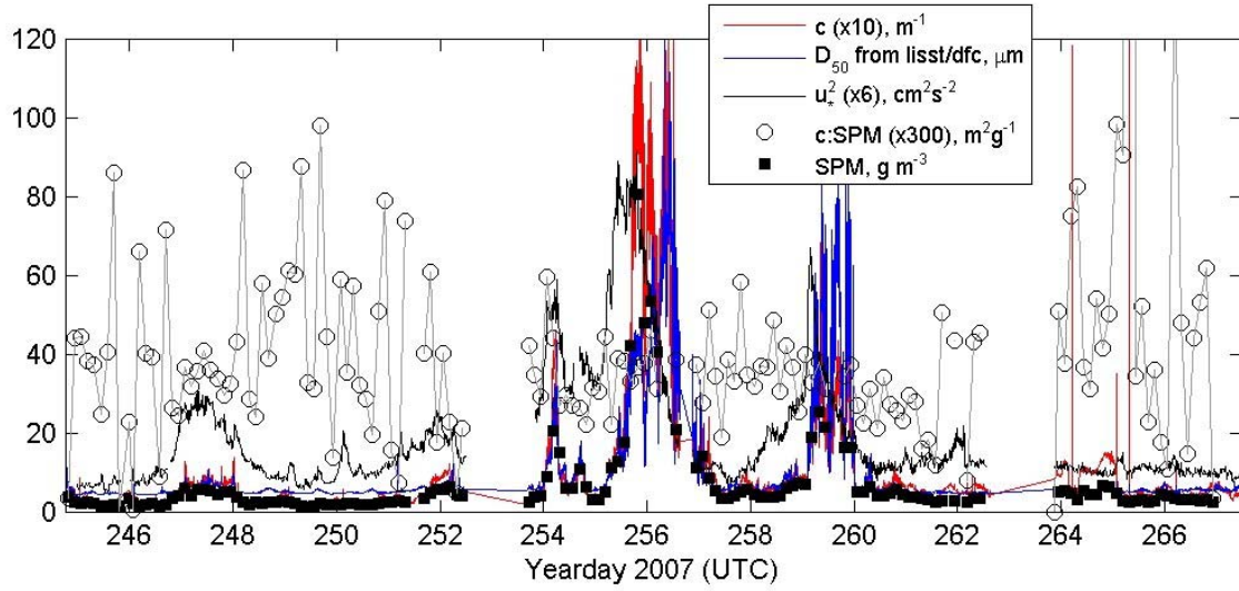
Figure 1. Time series of optical attenuation ( c ), median particle size ( D_{50} ), the square of shear velocity ( u_{*}^2 ), which is proportional to bottom stress, suspended particulate mass (SPM), and the mass normalized attenuation coefficient, which is the slope of the linear relationship between attenuation and SPM ( c:SPM ). When bottom stress is low, the mass normalized attenuation coefficient is variable, but when bottom stress is high, its value stabilizes, despite variability in particle size.
