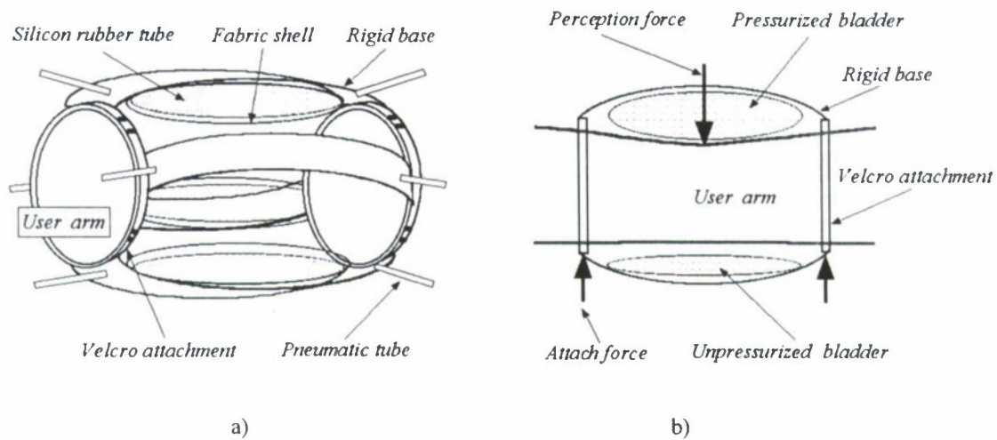
Figure 4: Illustration of the pneumatic actuator: a) set of 4 bladders, b) forces distribution.
