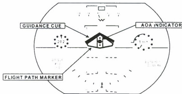
Figure 9: HMD Approach-Path Command Guidance
