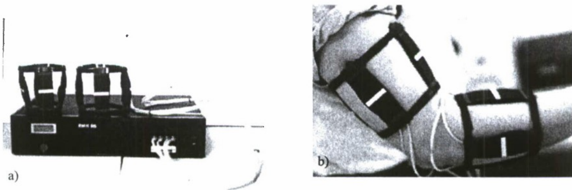
Figure 5: Elbow interface: a) controller unit, b) user's arm wearing the interface unit.
