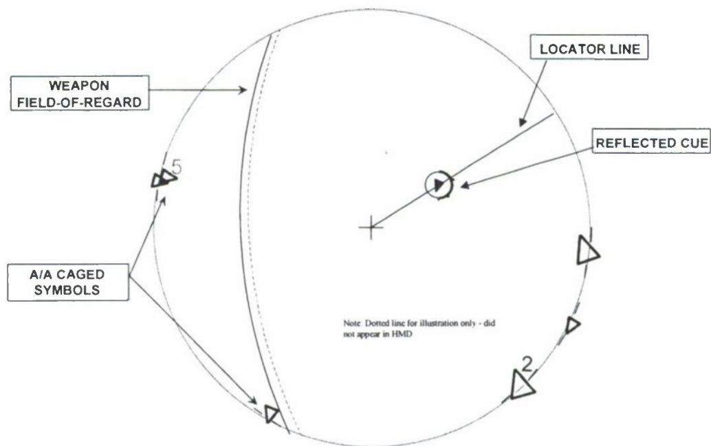
Figure 5: Advanced A/A Symbolology
