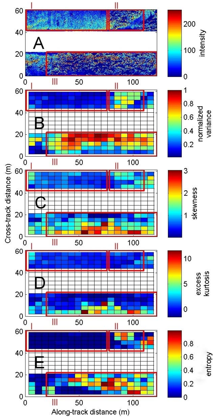
Figure 2 – Statistical analysis of sidescan image from figure 6. Panels show (as labeled): intensity, variance, skewness, kurtosis and entropy (respectively). Regions I, II and III correspond to sand, sand/coral and coral as identified in figure 6.
