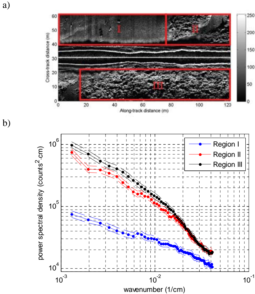
Figure 1 – a) Sample AUV sidescan image from survey at KN with 3 regions identified, corresponding to I: sand, II: mixed sand/coral, III: coral. b) acoustic intensity power spectral density from 3 regions identified in (a).
