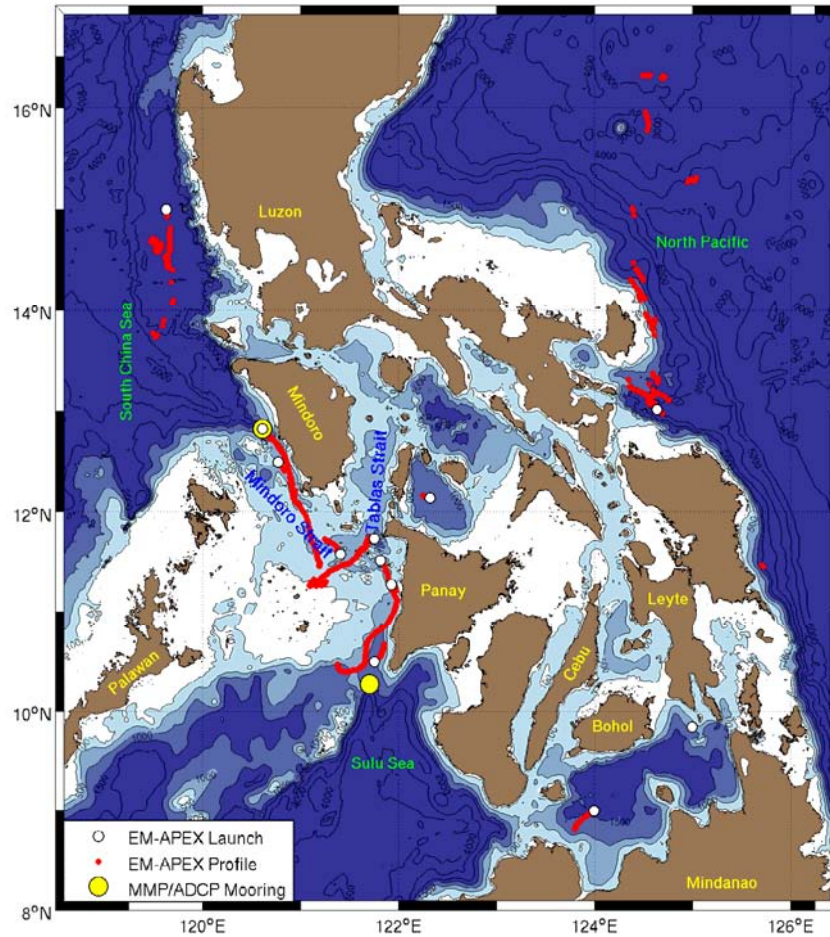
Figure 1: Locations of profiling moorings (yellow circles) and EM-APEX measurements (red dots) in the Philippine Archipelago. Mooring MP1 is at the northern (South China Sea) end of Mindoro Strait, and MP2 is at the southern (Sulu Sea) end. Shading indicates water deeper than 100m, 200m, 500m, and 1500m.
