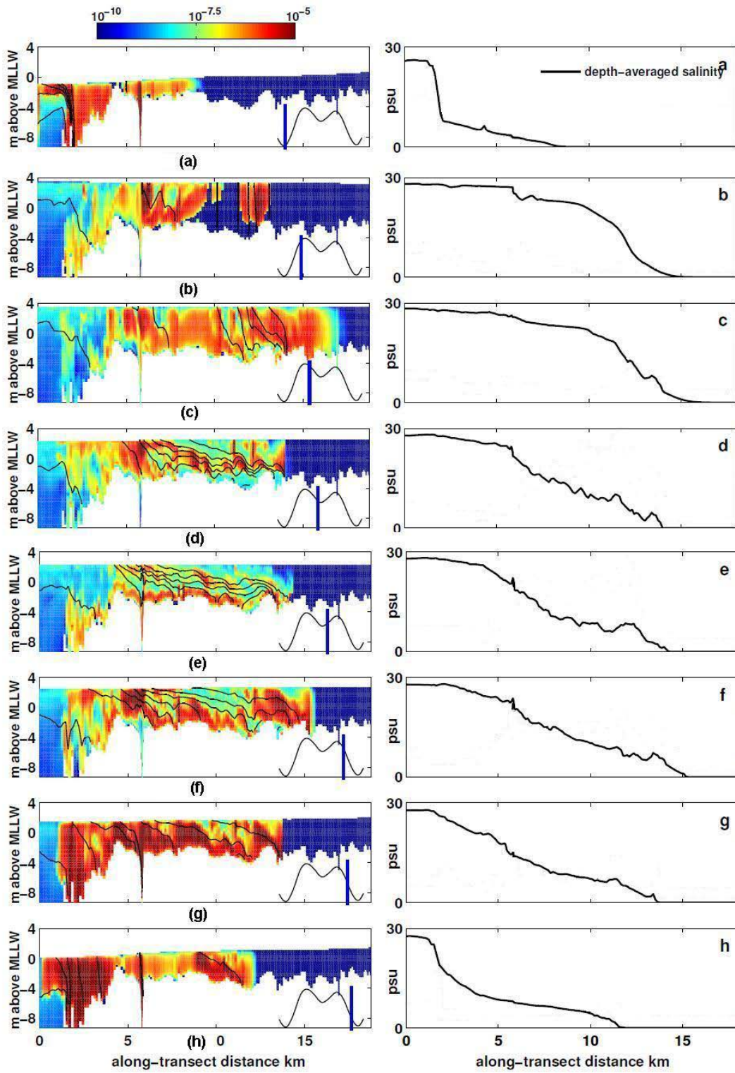
Figure E3: Buoyancy fluxes with salinity contours (left) and depth-averaged salinity along transect E-E' at different stages of a tidal cycle.
