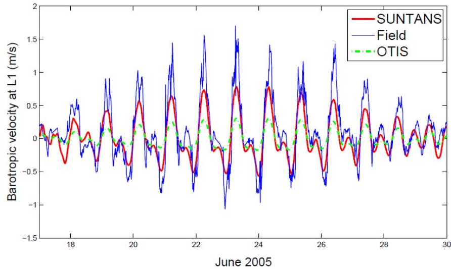
Figure 5: Comparison of barotropic currents at mooring L1 from observations (blue solid thin line), SUNTANS (red solid thick line) and OTIS (green dashed line) during June 17 to June 30, 2005. Positive currents indicate ebb tide towards the Pacific Ocean. The observed currents are the average over the water column extending from -450 m to -380 m.
