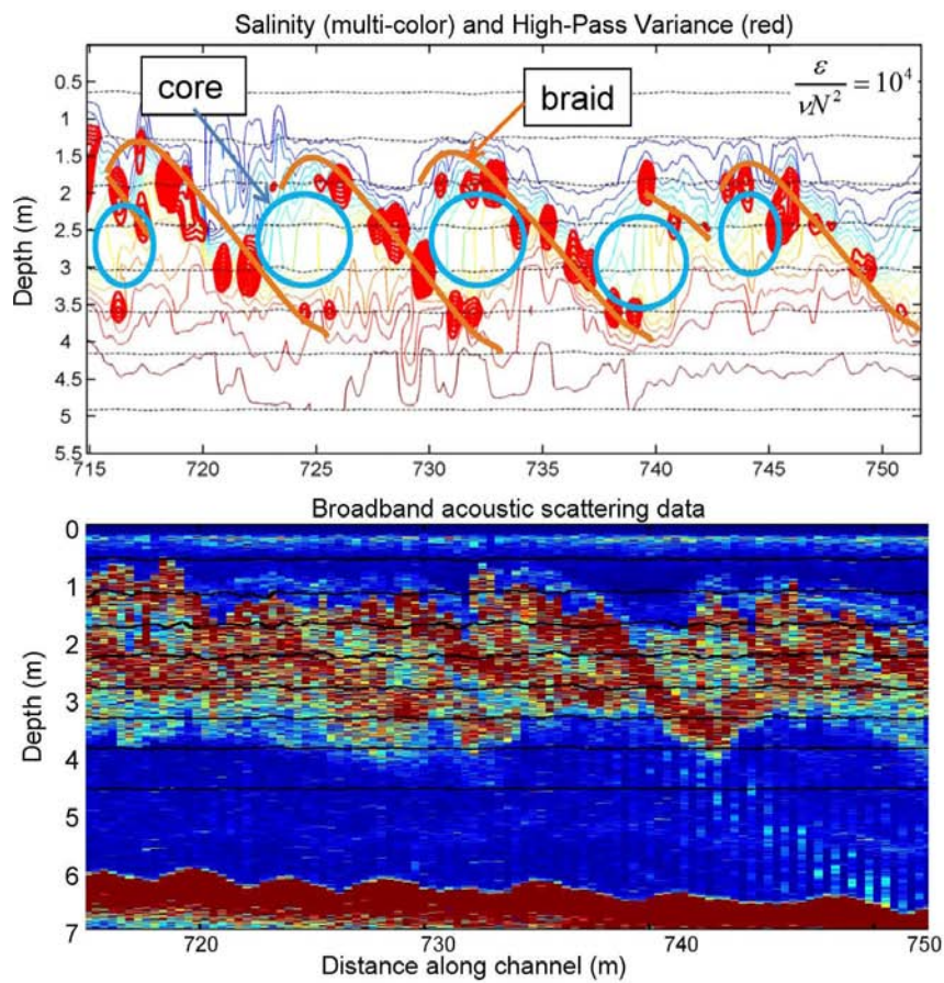
Figure 5. Coincident measurements of broadband acoustic scattering and salinity variance on similar scales, and the interpretation of these measurements.
