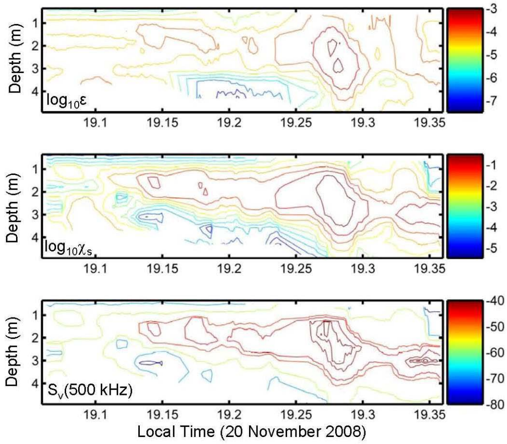
Figure 4. Measured dissipation rates and scalar variance in CT River in November 2008. Predictions of acoustic scattering at 500 kHz based on these measurements.
