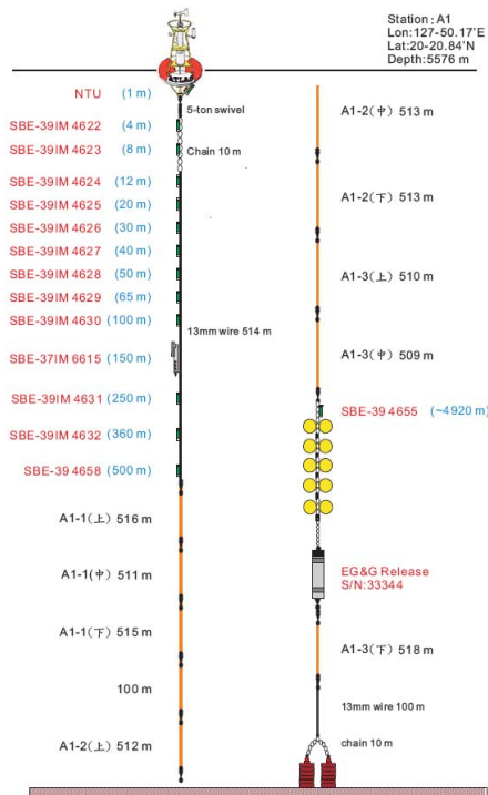
Figure 1. Schematic diagram of mooring A1 and photo of ITOP buoy. Moorings A2 and A3 are similar to that of A1.
