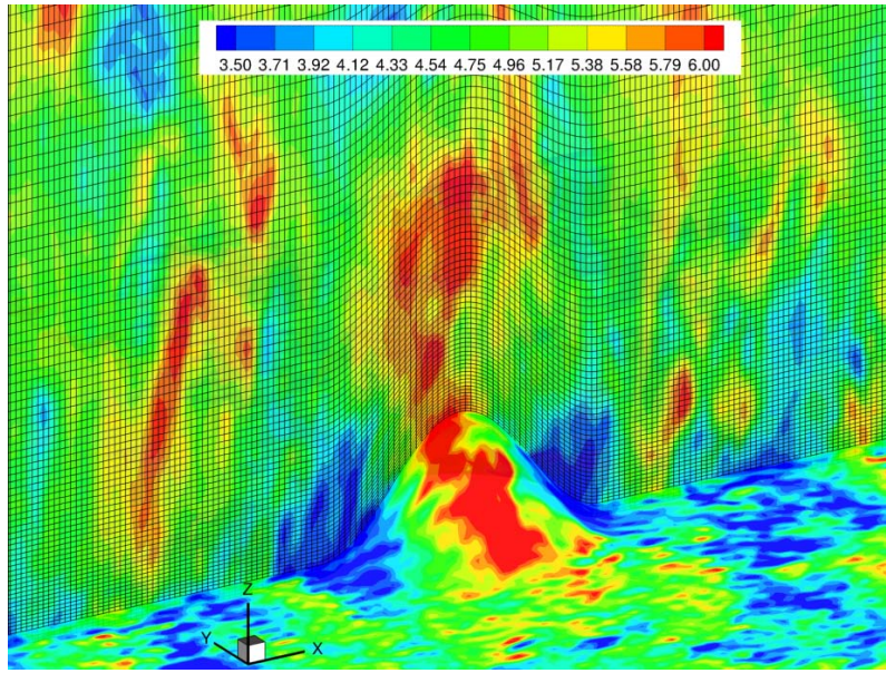
Figure 3: The turbulent wind field ( u -component) around and above an isolated hill in a mixed convective-shear driven atmospheric boundary layer - surface heat flux Q_* = 0.05 \text{ K m s}^{-1} and geostrophic wind U_g = 5 \text{ m s}^{-1} . The 3D cosine shaped hill is 50 m tall. Notice the wind speedup over the crest and side of the hill with u/U_g > 1.2 . The color bar at the top of the figure is in units of \text{m s}^{-1} . This simulation employs 256 \times 256 \times 128 gridpoints and demonstrates that the LES algorithm is capable of simulating turbulent flow above general topography.
