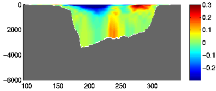
Figure 9: Snapshot of a cross-vertical section (89°W) of baroclinic meridional velocities. The abscissa is index of the model and ordinate is depth in meters.
