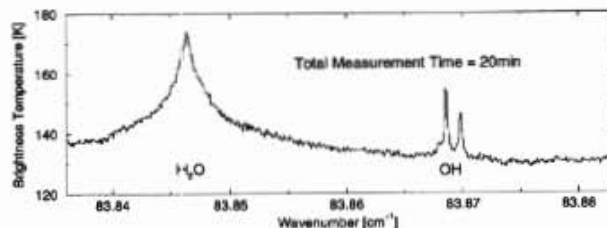
Figure 1. Calibrated spectrum measured during the THOMAS/MAHRSI campaign in August 1997.
