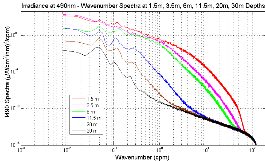
Figure 5. Shown is the wave number spectra at six depths for irradiance at 490 nm observed on Sep 20, 2009. Westerly winds were about 6 m/s and solar insolation varied from 650 to 850 W m^{-2} during the observation. The fluctuations at shorter wave numbers decrease rapidly with depth.
