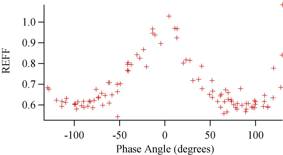
Figure 10 Flocculent sample, 65 deg incidence, REFF vs Phase Angle
