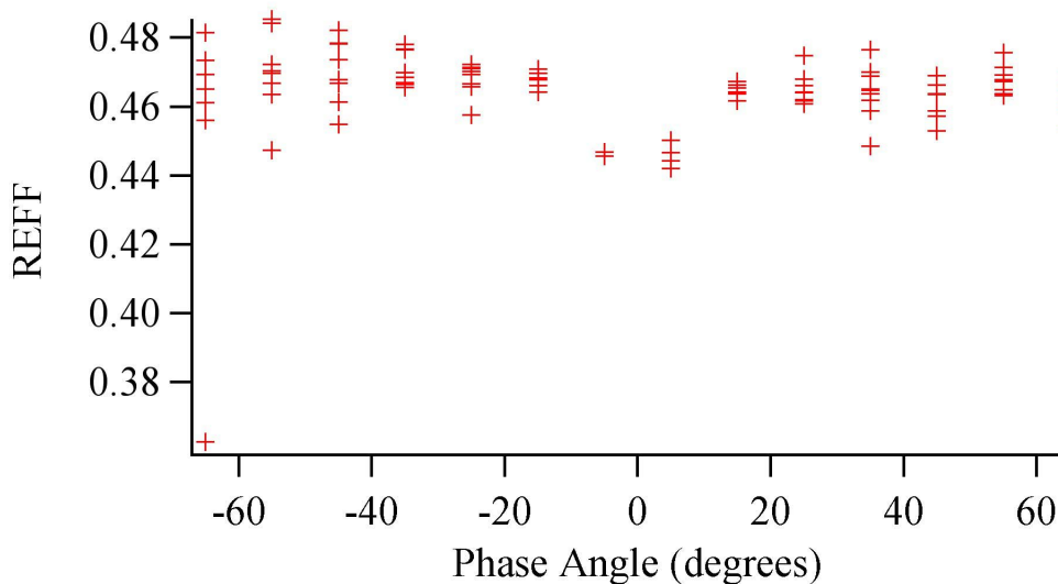
Figure 7 Quartz Sand, 0 degree incidence, REFF vs Phase Angle
