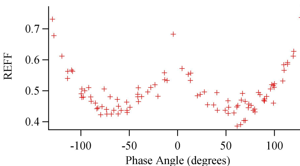
Figure 8 Quartz sand, 65 degree incidence, REFF vs Phase Angle
