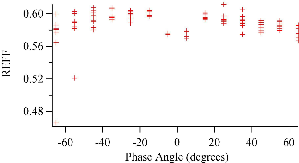
Figure 5 Ooid sample, 0 deg incidence, REFF vs Phase Angle
