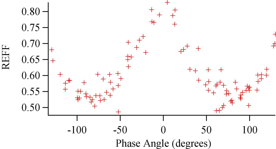
Figure 6 Ooid sample, 65 degree incidence, REFF vs Phase Angle
