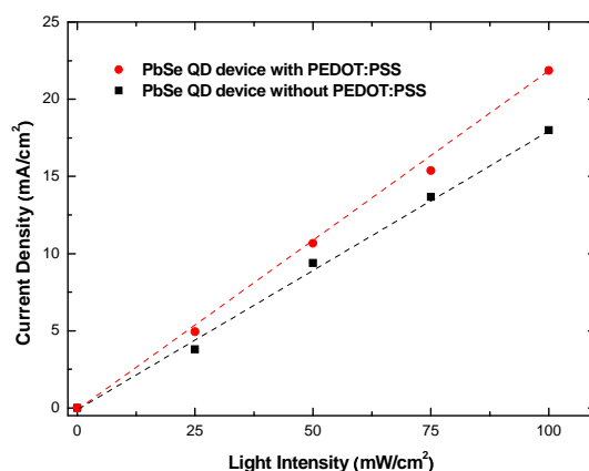
Figure 5. Photocurrent density ( J_{sc} ) plotted with respect to the intensity of solar light for the PbSe QD device prepared with and without a PEDOT:PSS layer.
