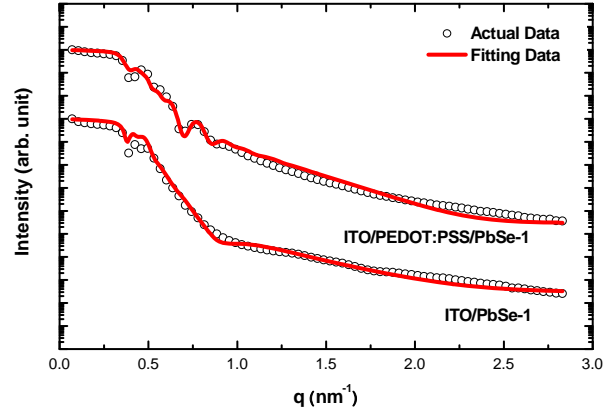
Figure 2. (b) Synchrotron X-ray reflectance for structures incorporating PbSe QD layers, prepared with and without a PEDOT:PSS thin layer.
