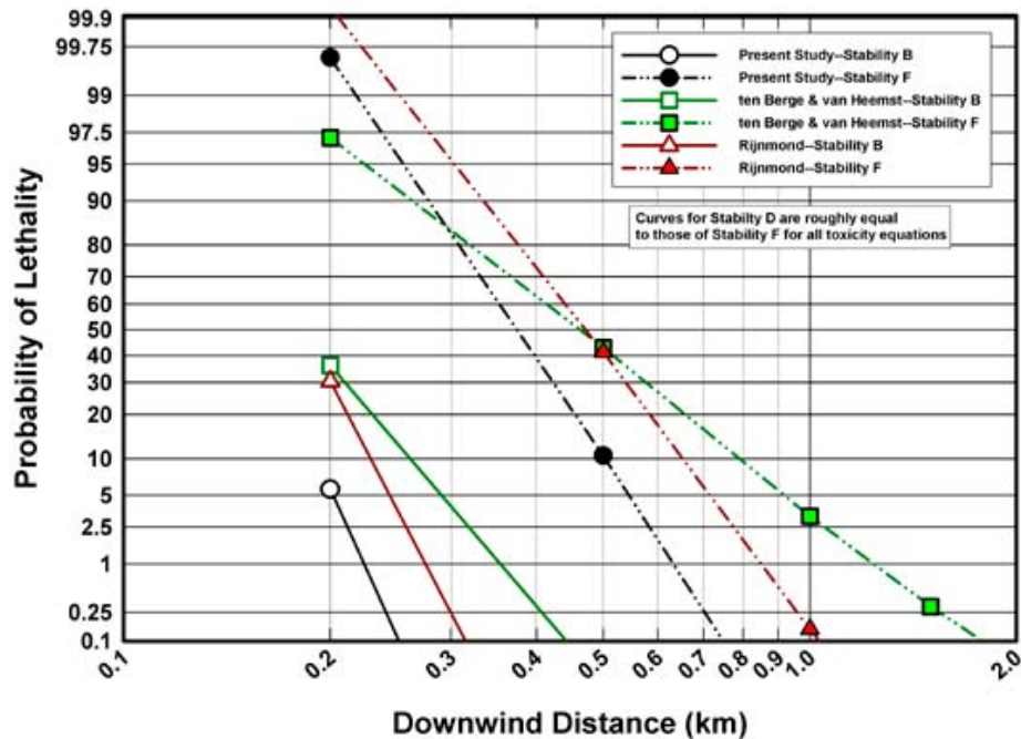
Figure 7-8. Probability of lethality versus downwind distance for several human chlorine lethality estimates (Pasquill Stability Categories B and F)
