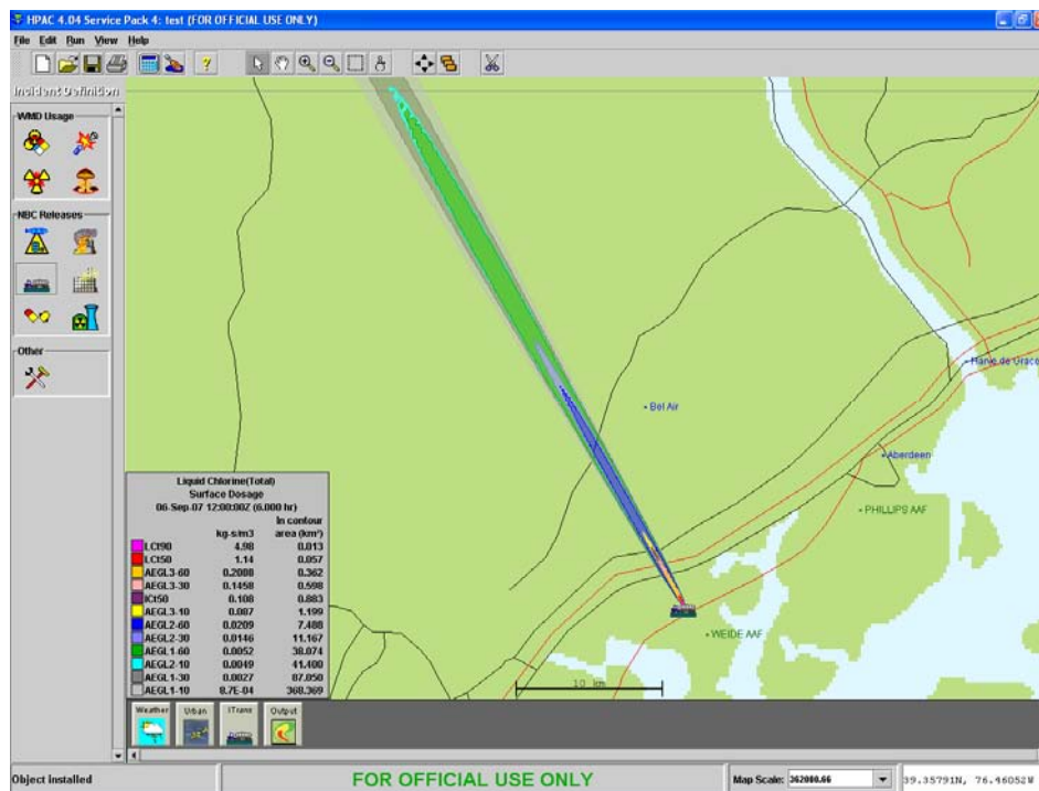
Figure I-5. HPAC plumes (low resolution) for moderate wind (5 m/s), cloudy day, “neutral” condition (Pasquill Category D)
