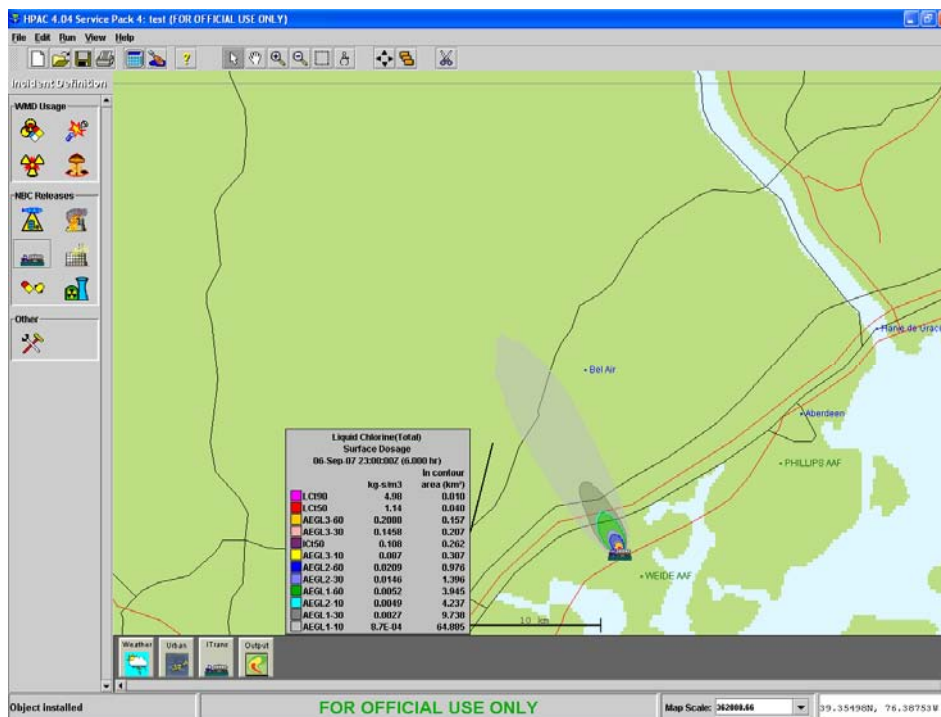
Figure I-6. HPAC plumes (low resolution) for low wind (2 m/s), clear sky, daytime (2 p.m.), “unstable” condition (Pasquill Category B)
