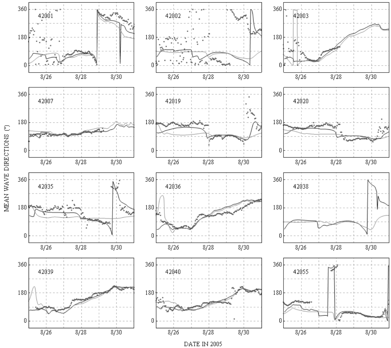
Figure 7: Mean wave directions ( ^{\circ} ), measured clockwise from geographic north, during Hurricane Katrina at 12 NDBC buoys. The measured data is shown with black dots, the modeled SWAN results are shown with black lines, and the modeled WAM results are shown with gray lines.
