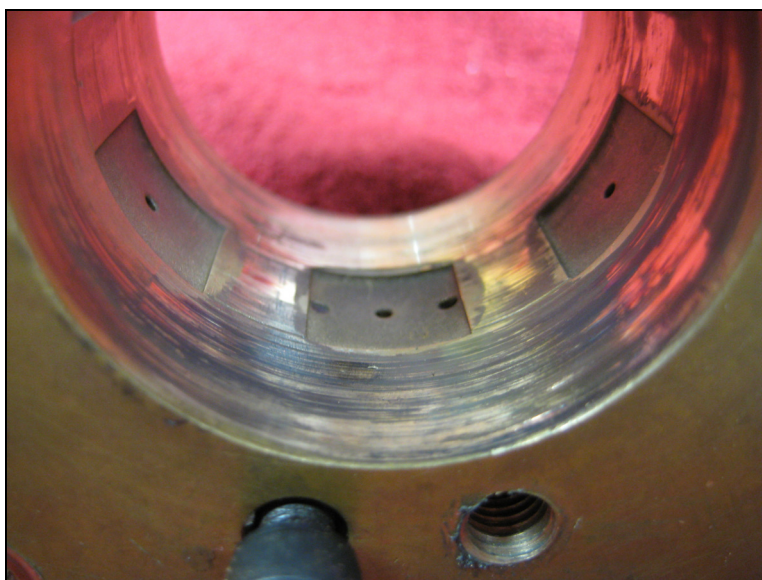
Fig. 39 Burnishing of the bearing with applied unit load LOR direction
