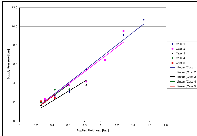
Fig. 22 Hydrostatic lift-off supply pressure versus applied unit load for the LOR cases
