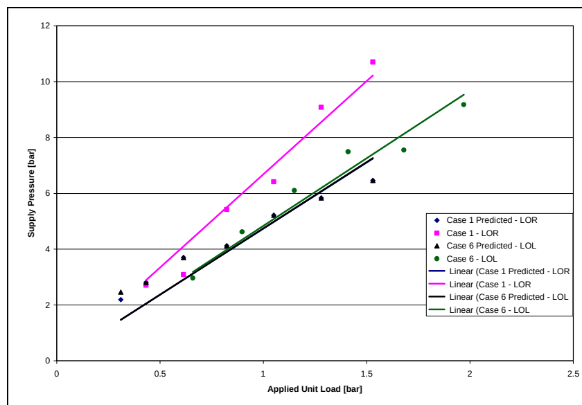
Fig. 28 Predicted and actual hydrostatic lift-off supply pressure versus applied unit load for cases 1 (LOR) and 6 (LOL).
