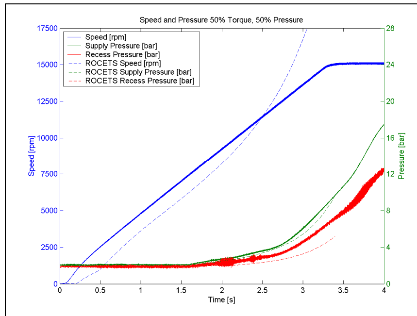
Fig. 9 Comparison between ROCETS data and start-transient test
