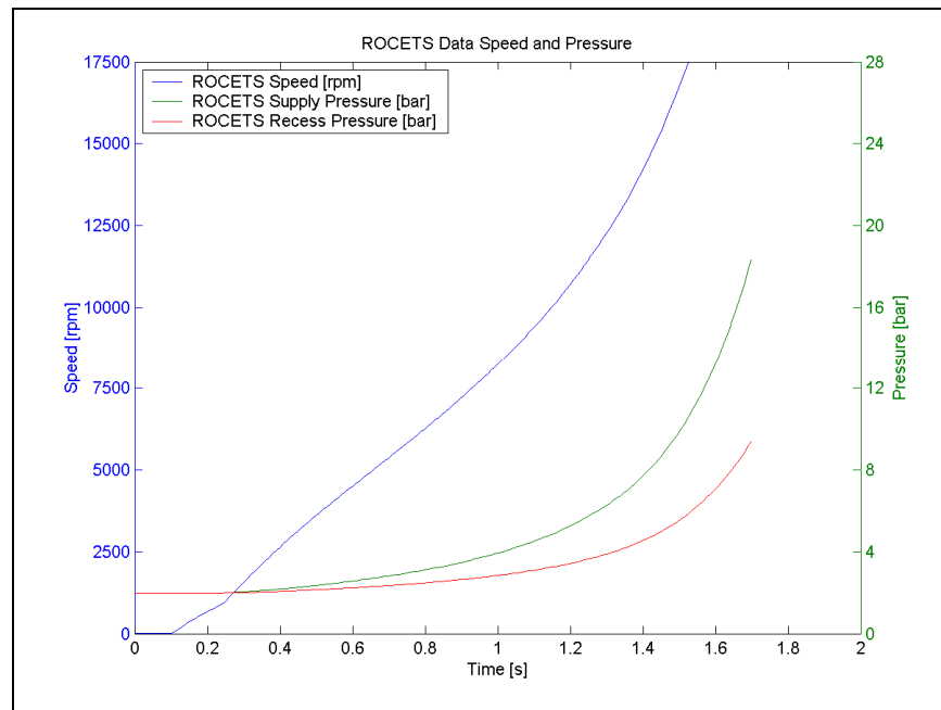
Fig. 8 NGST ROCETS data of a next generation turbo-pump provided for replication
