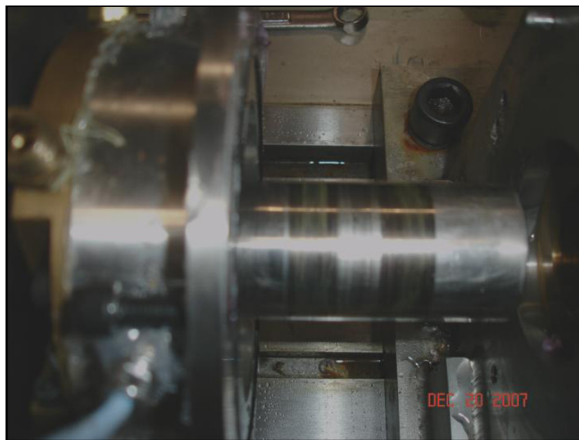
Fig. 34 Burnishing of the rotor observed after testing by Borchard [5]
