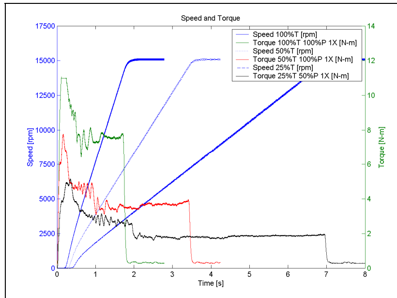
Fig. 30 Drive torque for varying ramp rates
