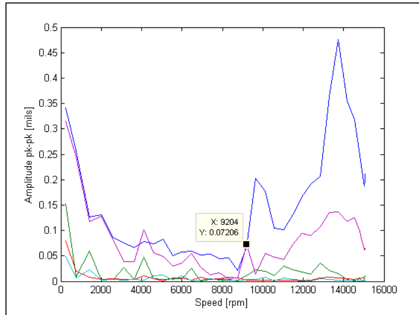
Fig. 29 Forward and backward amplitude for the 100% Torque-100% Pressure, 6X static unit load, LOP
