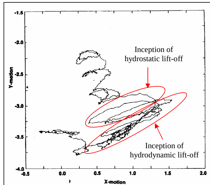
Fig. 1 Orbit plots showing hydrodynamic and hydrostatic lift-off from Scharrer et al. [3]
