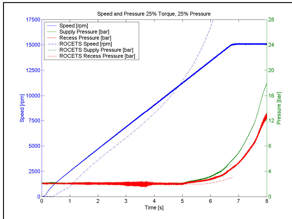
Fig. 46 Comparison between ROCETS data and start-transient test 25% Torque-25% Pressure
