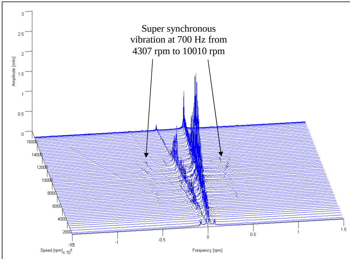
Fig. 58 Double sided waterfall plot for outboard proximity probes for 50% Torque-50% Pressure 4X linear unit load.
