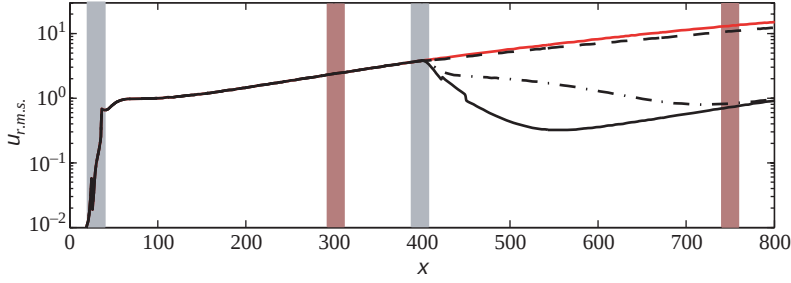
FIGURE 15. The r.m.s. values of the uncontrolled system (red line), cheap controller (solid black), intermediate controller (dashed-dotted line) and expensive controller (dashed line). The grey bar represent the size (defined as 99 % of the spatial support) and the location of the two inputs, whereas the red bars correspond to the two outputs.
