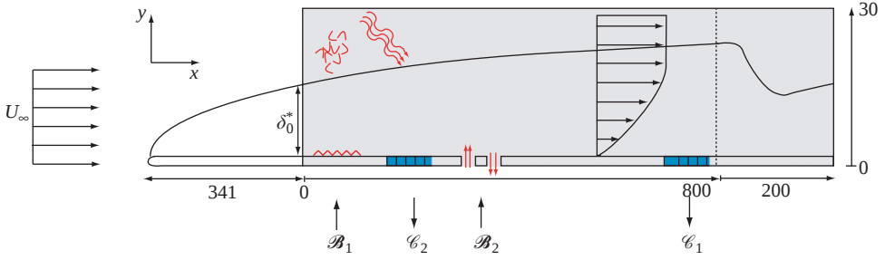
FIGURE 1. Conceptual figure of the input–output configuration used for the control of perturbations in a two-dimensional flat-plate geometry. The computational domain \Omega = (0, L_x) \times (0, L_y) , shown by the grey region, extends from x=0 to x=1000 with the fringe region starting at x=800 . The first input \mathcal{B}_1 , located at (x_w, y_w) = (35, 1) , models the initial receptivity phase, where disturbances are induced by free stream turbulence, acoustic waves or wall roughness. The actuator \mathcal{B}_2 provides a means to manipulate the flow, in this case by a localized volume forcing, and is centred at (x_u, y_u) = (400, 1) . Two sensors \mathcal{C}_1 and \mathcal{C}_2 are located at (x_v, y_v) = (300, 1) and (x_z, y_z) = (750, 1) respectively. The upstream measurements are used to estimate the incoming perturbations, while the downstream sensor quantifies the effect of the control. Note that in this work all the inputs and outputs are Gaussian functions given by (2.14).
