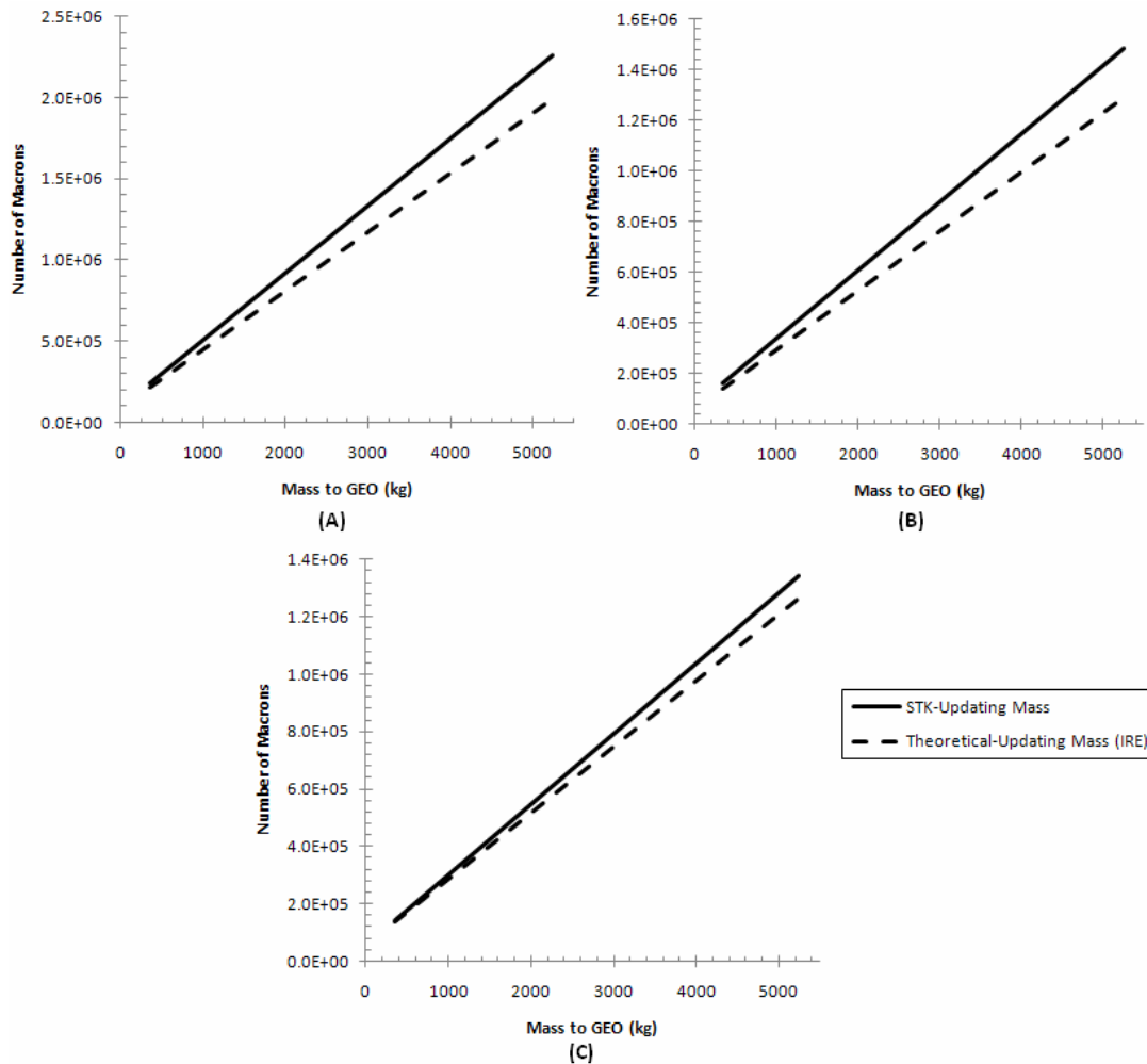
Figure 7. Number of macrons required to transfer a given mass from LEO to GEO. (A) 1g, 7.07km/s (B) 10g, 2.24km/s (C) 1g, 10km/s
