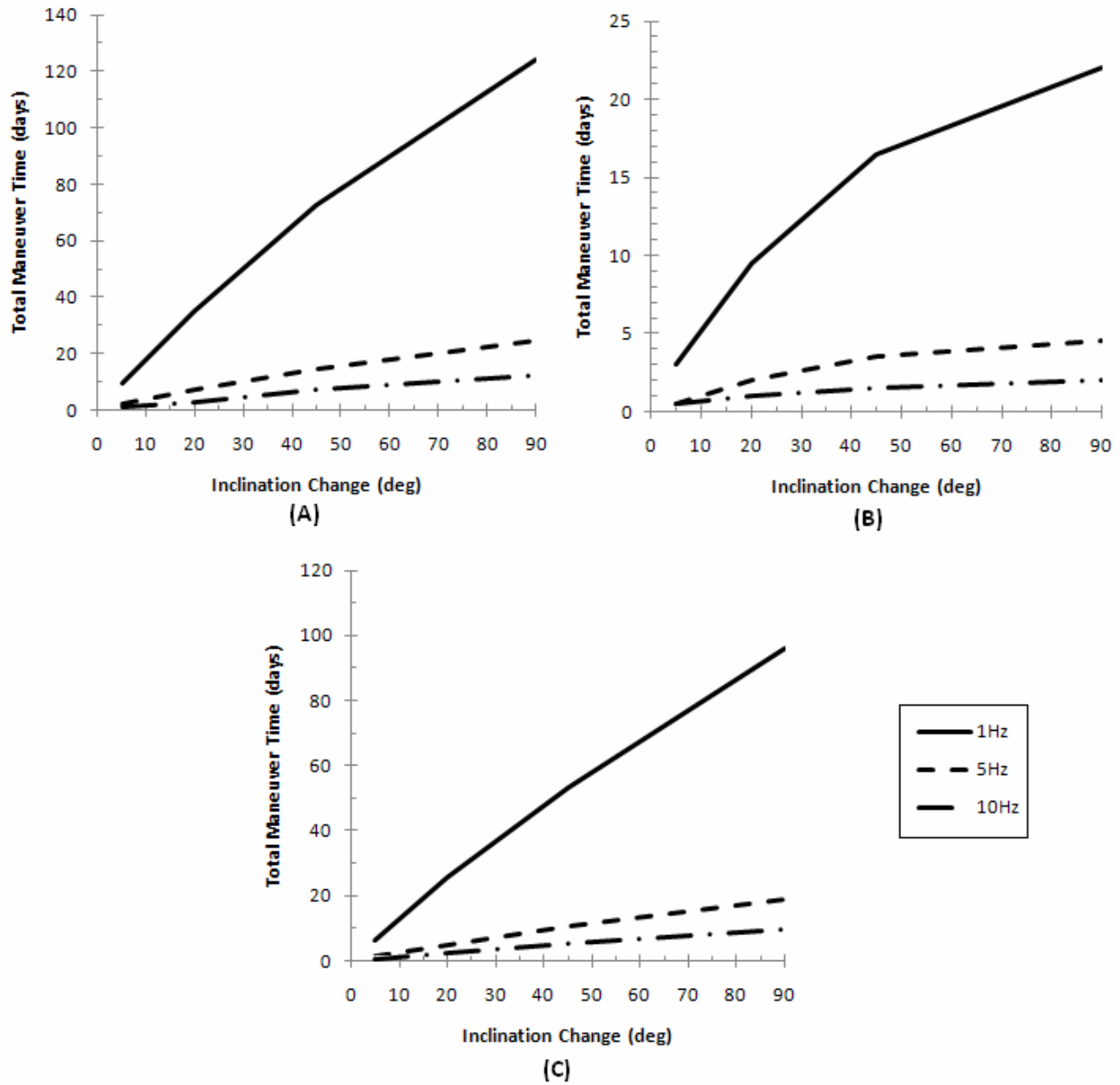
Figure 10. Total time to complete a GEO inclination change as a function of repetition rate. (A) 1g, 7.07km/s (B) 10g, 2.24km/s (C) 1g, 10km/s
