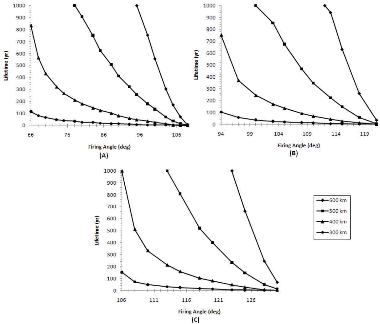
Figure 4. EOVS code orbital lifetimes versus macron firing angles as a function of firing altitude. (A) 1g, 7.07km/s (B) 10g, 2.24km/s (C) 1g, 10km/s
