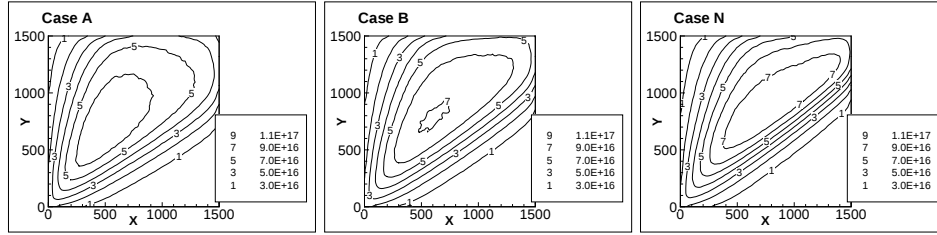
FIGURE 3. Total number density ( m^{-3} ) fields at f_i values of 0.0, 0.1, and 0.5.
