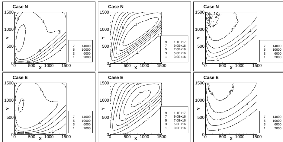
FIGURE 4. From left to right: overall translational temperature (K), total number density ( m^{-3} ), and CO rotational temperature (K) fields at \omega values of 0.75 and 0.90. The top row corresponds to \omega of 0.75; the bottom is \omega of 0.90.
