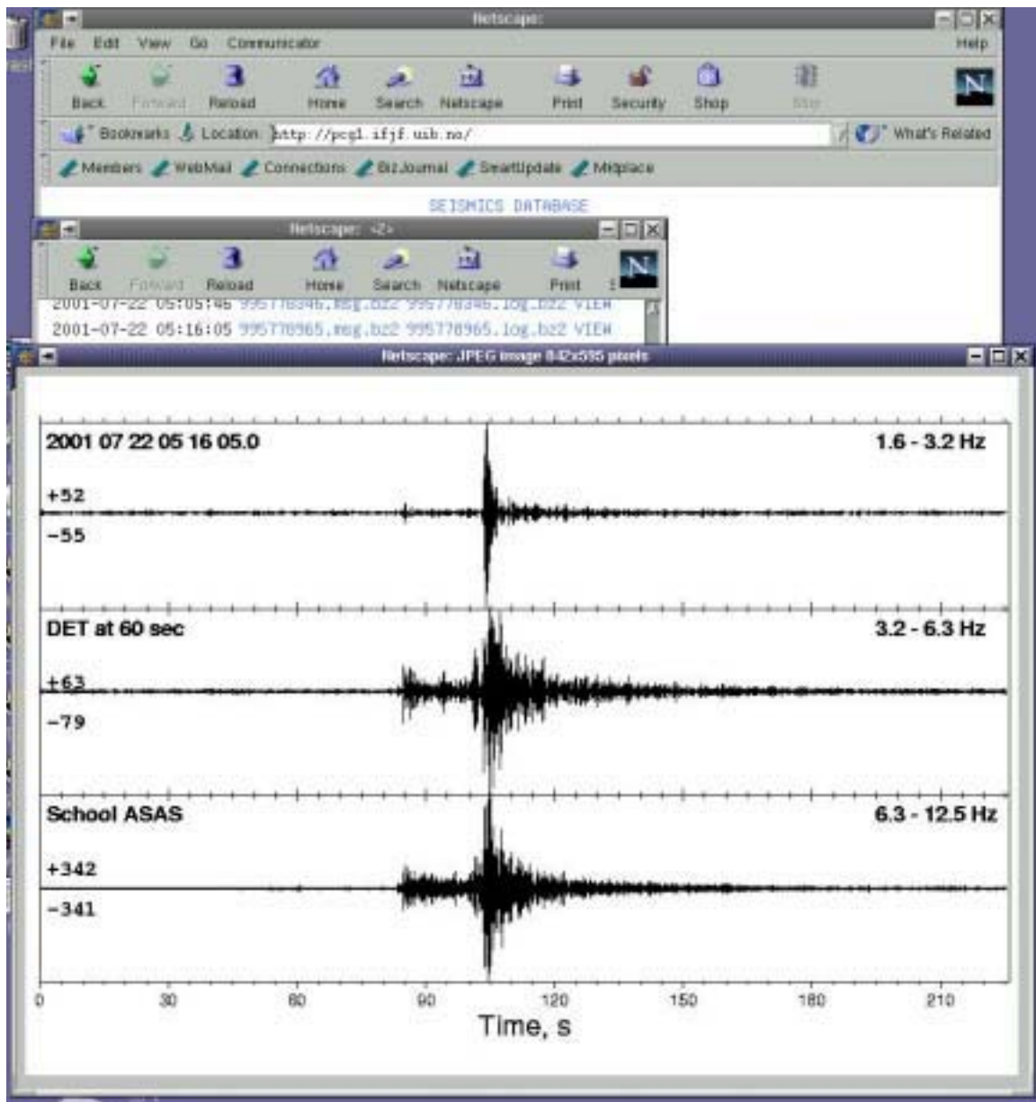
Figure 3. Viewing 'school station' recordings on Internet http://pcg1.ifjf.uib.no/ . The SEISMICS DATABASE appears and a click gives station choice - see insert in Fig. 1. A click then gives options of date for viewing; Year/Month/Day. Then the daily detections with view options appear; a click here produce more than 200 seconds of Z-comp. traces in the respective 3 filter bands of the detector. In near future detection logs would also be available for individual stations and multistation detections which will facilitate event selections significantly for school participants. Our efficient 2D detector detects much of garbage signals of very local origin which will be automatically removed from log listings. Waveform data access requires password.
