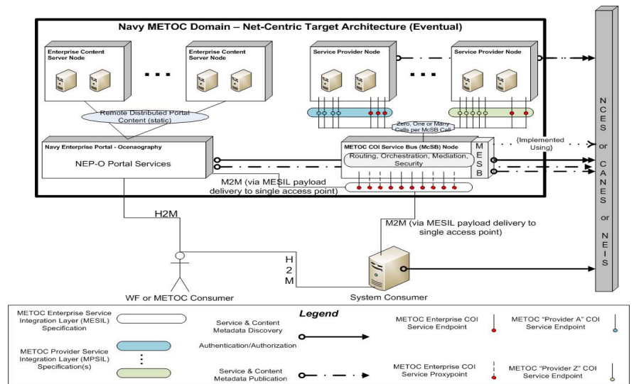
Figure 7 - Net-Centric Target Architecture
