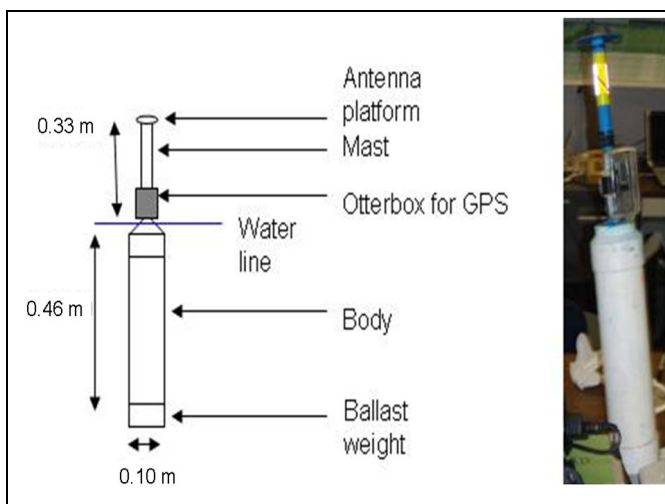
Fig. 1 Schematic of the GPS-equipped river drifter and photograph.
