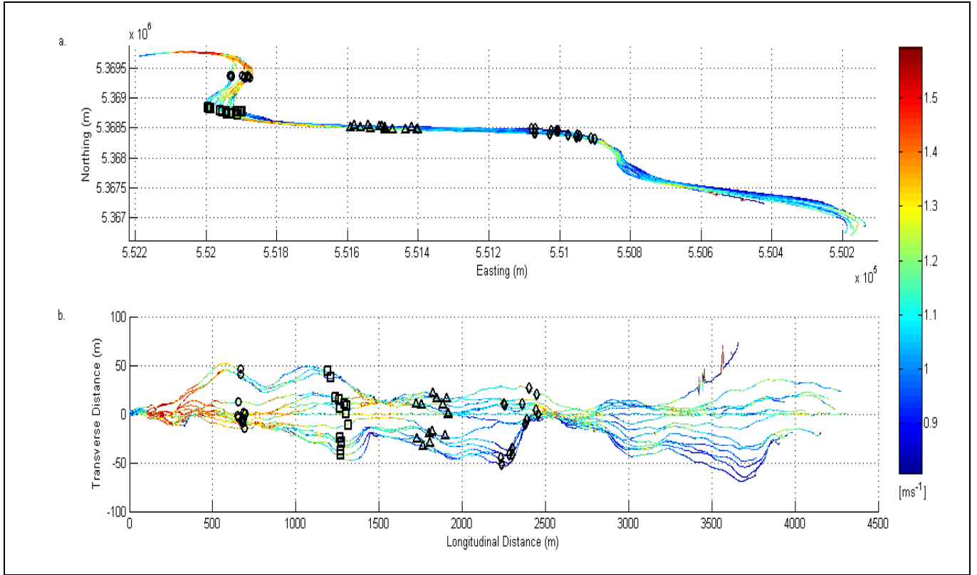
Fig. 3: Upper Skagit deployment coordinate transform: (a) geographic coordinates, (b) river-fitted local coordinate frame utilizing Legleiter and Kyriadkdis (2007) technique. Symbols represent the position of the drifters at 500 (circle), 1000 (square), 1500 (triangle) and 2000 (diamond) seconds after release. Colorbar plotted on the right, where color represents drifter speed.
