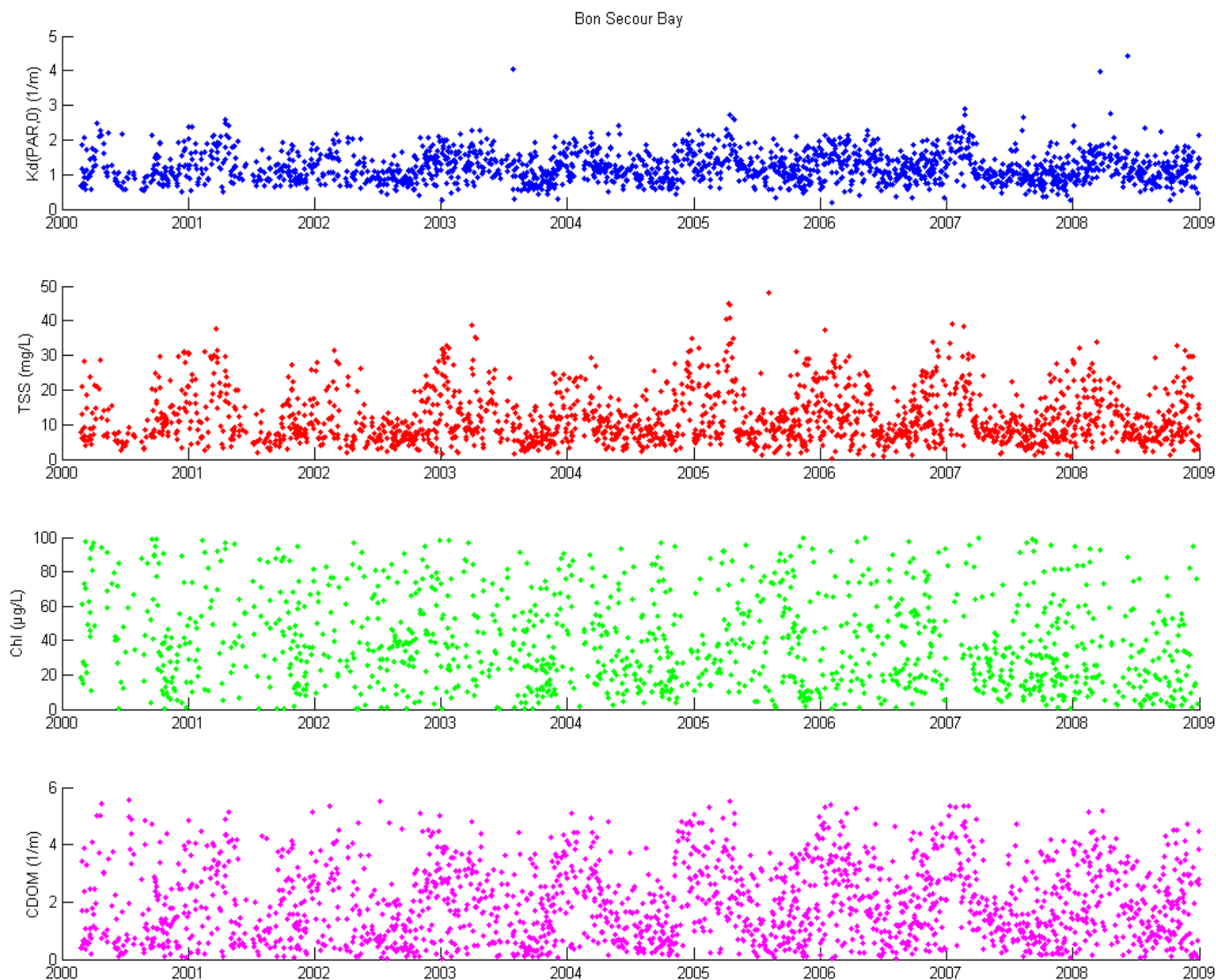
Fig. 5 Time series of water clarity parameters retrieved from MODIS remote sensing measurements for the Bon Secour Bay area.
