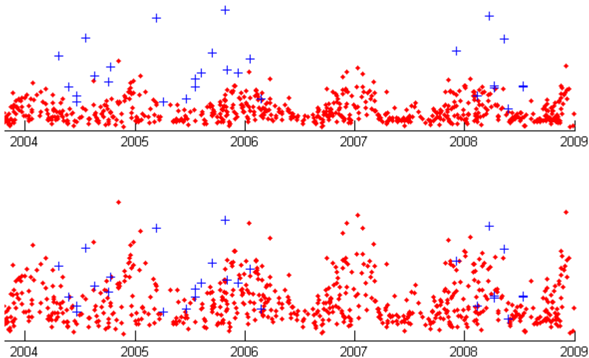
Fig. 4. Comparison between subsets of TSS time series generated from MODIS data (dots) using (4) with b/b_0 = 50 (top) and b/b_0 = 100 (bottom) and the surface water monitoring measurements (crosses) collected by ADEM (2004-2006) and MSU (2007-2008) at the MB3a sampling station. TSS scale and units are the same as in Fig 3.
