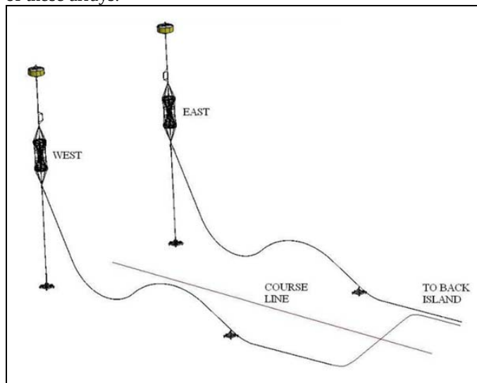
Figure 2 – SEAFAC HGMS Arrays
