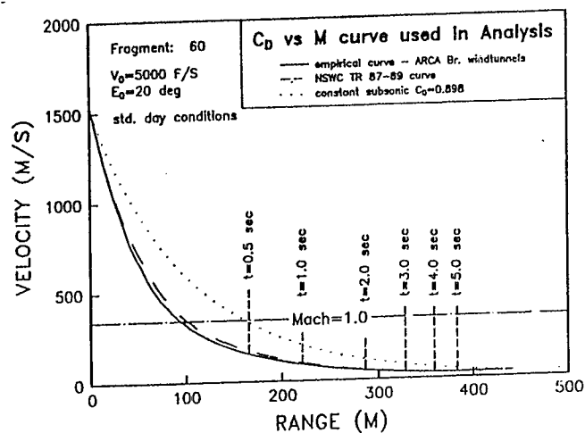
Fig 15. Computed Velocity Decay With Range
