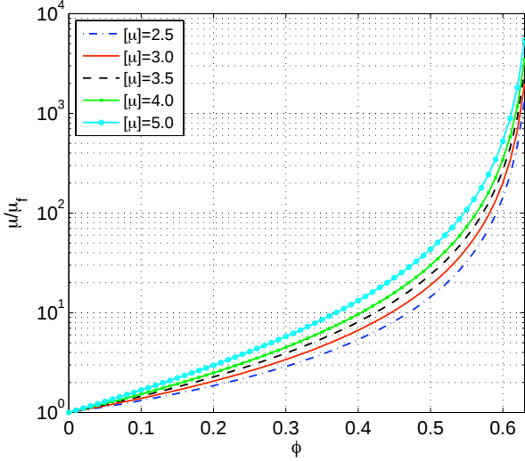
Fig. 2. The scaled effective viscosity (4) resulting from varying intrinsic viscosities, [\mu] , versus volume fraction of sediment, \phi .
