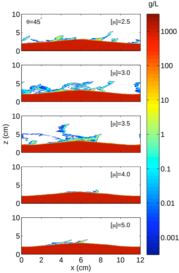
Fig. 4. Suspended sediment concentration fields ensemble averaged over three wave periods at maximum flow acceleration ( \theta = 45^\circ ) for varying intrinsic viscosities.
