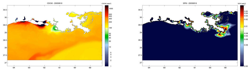
Fig. 8 Initial test run results for CDOM and suspended particulate matter (SPM) for June 18, 2003. The x-axis is degrees longitude and the y-axis is degrees North latitude.
