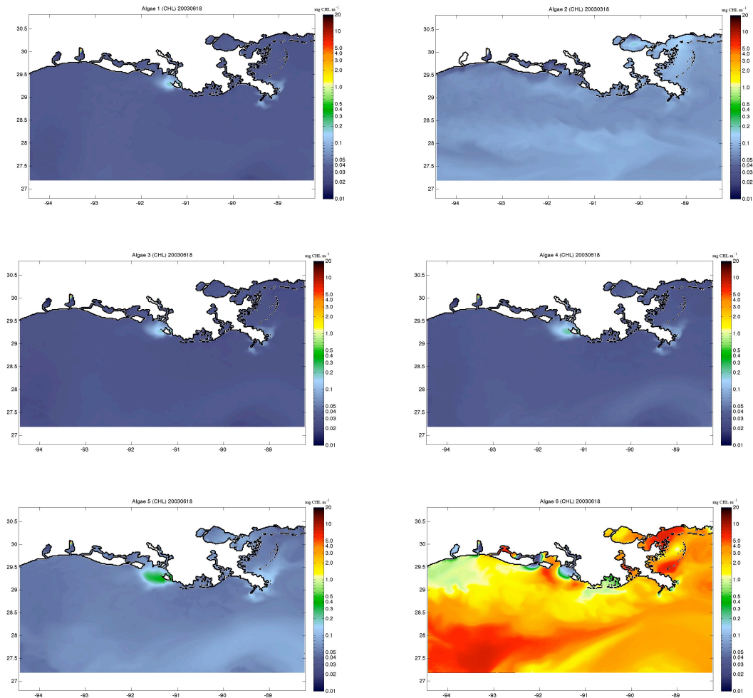
Fig. 7 Results for each of the phytoplankton (Algae 1-6) groups ( \text{mg Chl m}^{-3} ) from our initial test run of the coupled model (June 18, 2003). The x-axis is degrees longitude and the y-axis is degrees North latitude.
