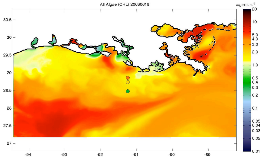
Fig. 6 Results for total phytoplankton chlorophyll ( \text{mg CHL m}^{-3} ) from our initial test run of the coupled model (x-axis is degrees longitude and y-axis is degrees North latitude). Colored circles represent in situ measurements. The date is June 18, 2003 for comparison with Fig. 2.
