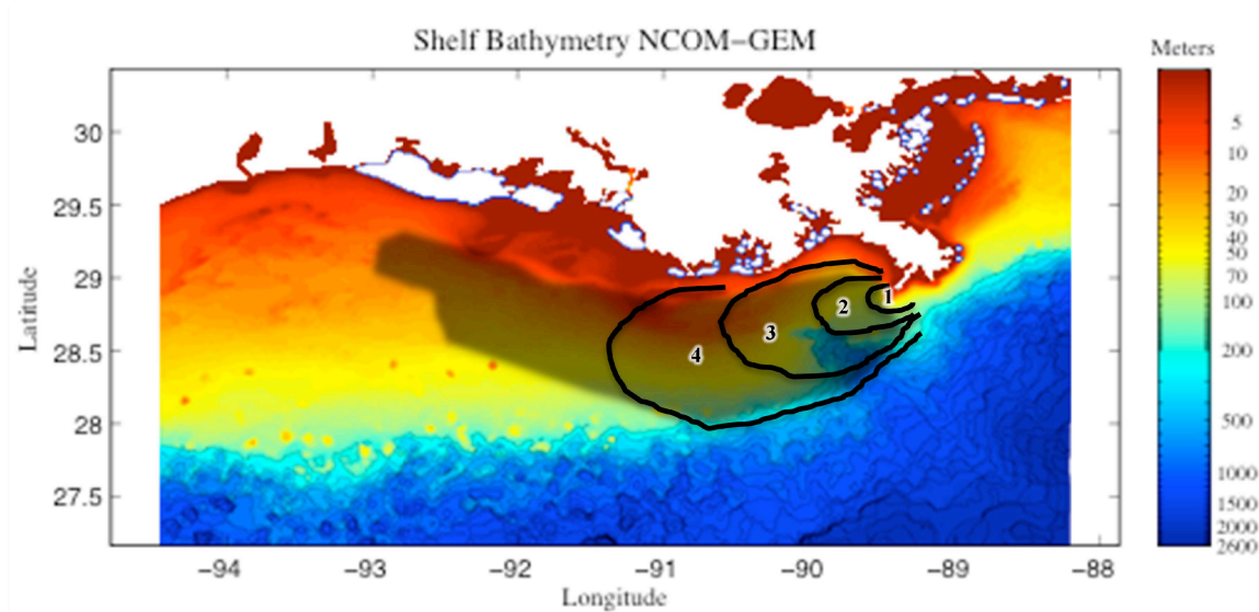
Fig. 1 Bathymetry of the Louisiana Shelf (m) with the hypoxia region depicted in gray. The four regions used in the ‘box model’ version of the biogeochemical model (see text) are also shown (1-4). This is the domain of the physical and coupled biogeochemical models.
