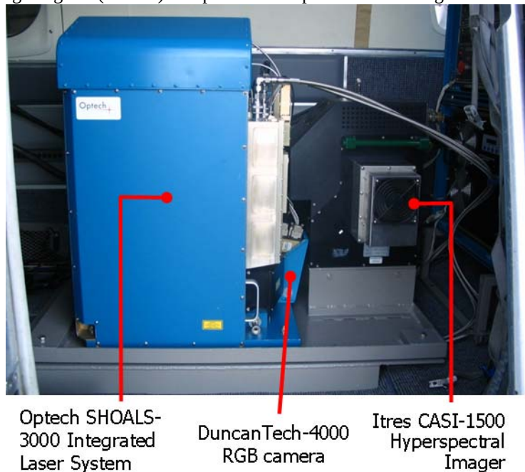
Fig. 1 Compact Hydrographic Airborne Rapid Total Survey (CHARTS) system.
