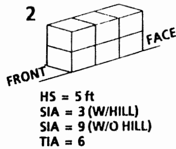
FIGURE 6 STACK CONFIGURATIONS KOREAN HILLSIDE BARRICADE: TAEGU: BUILDING 230 6 PALLETS MK 82: 6 BOMBS PER PALLET
