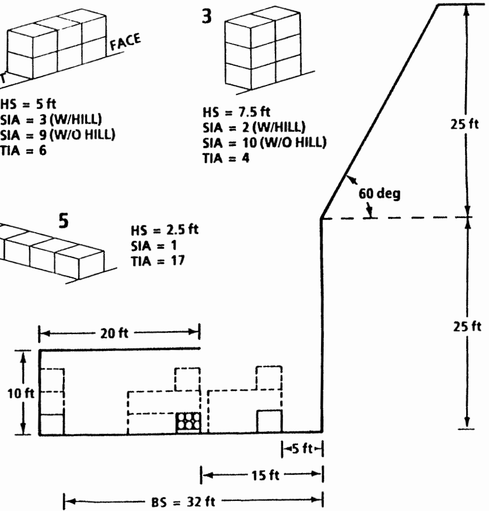
FIGURE 6 STACK CONFIGURATIONS KOREAN HILLSIDE BARRICADE: TAEGU: BUILDING 230 6 PALLETS MK 82: 6 BOMBS PER PALLET
