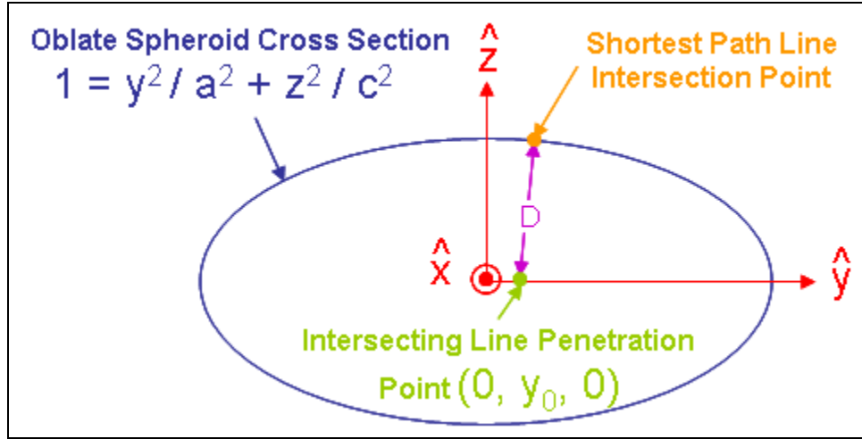
Figure 18. The y-z cross section of the oblate spheroid of figure 17.
