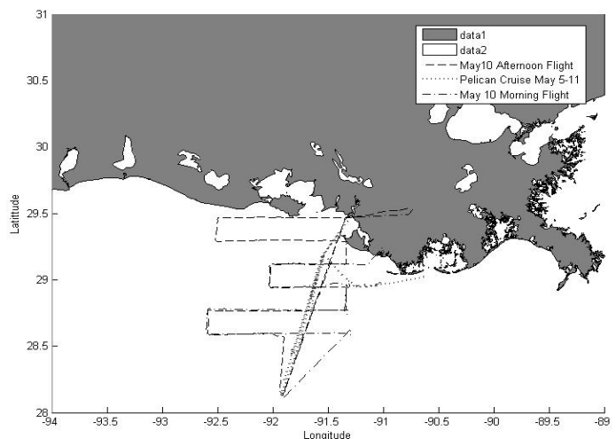
Figure 1. Entire flight tracks of aircraft and R/V Pelican May 2007
