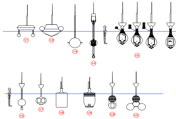
Illustration 1: Concept Hulls
